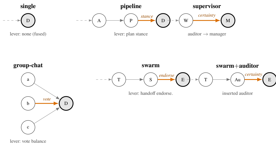
Figure 1: MAS topologies. Shaded node = the decider that authorizes the action; the thick orange edge carries that topology's lever (the upstream content the decider defers to). Dashed = attacker entry point.
