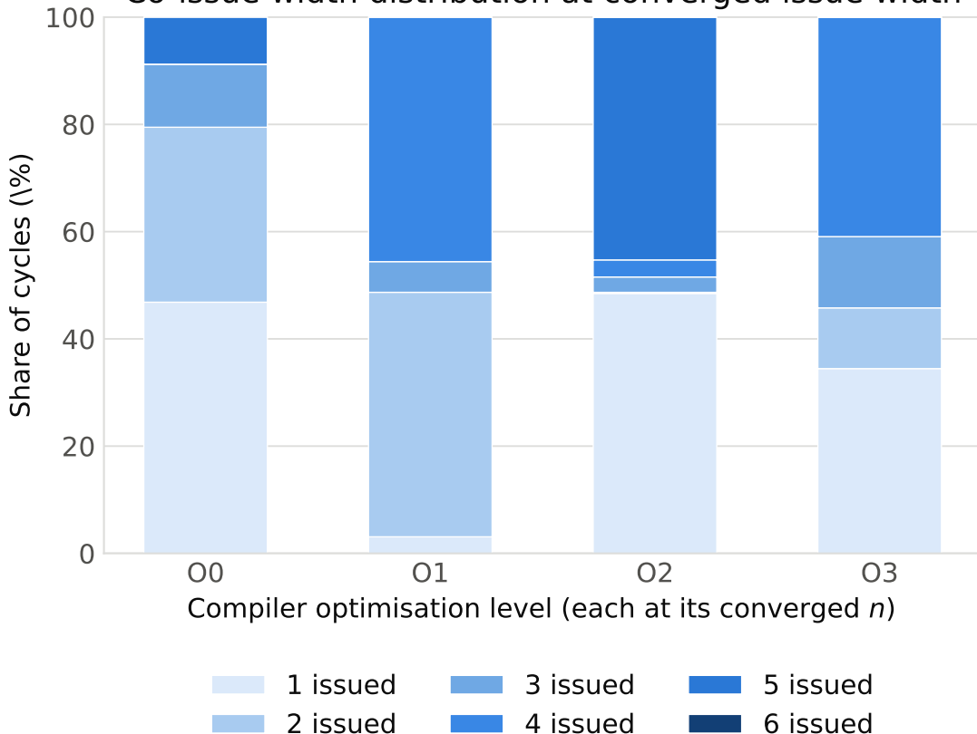
Co-issue width distribution at converged issue width
