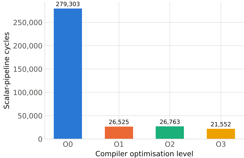
256×256 NPU matmul: cycles vs. optimisation level (issue width 1)
