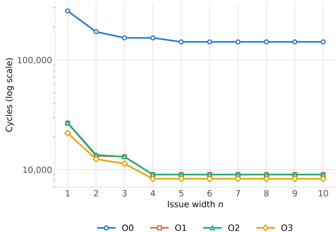
Cycles vs. superscalar issue width, by optimisation level
