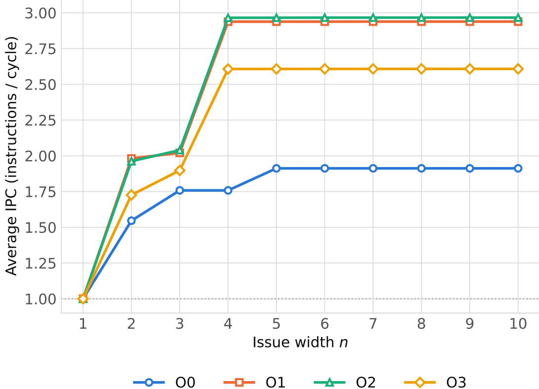
IPC vs. superscalar issue width, by optimisation level
