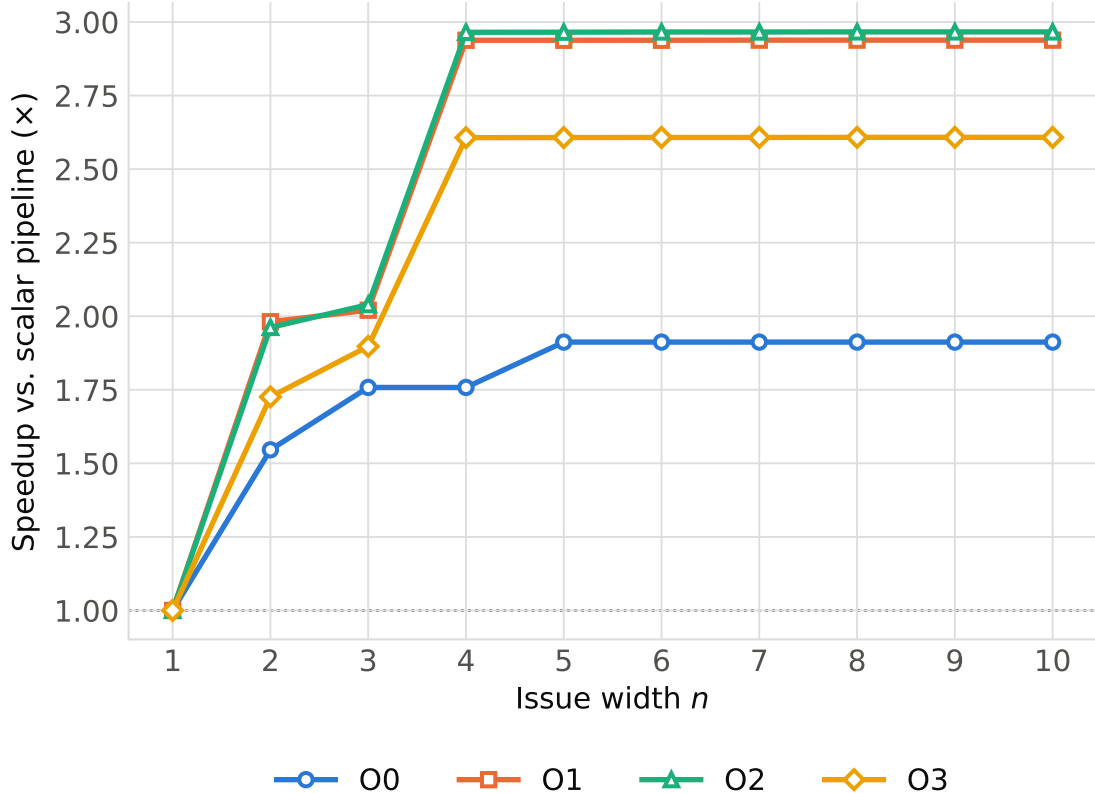
Speedup vs. superscalar issue width, by optimisation level
