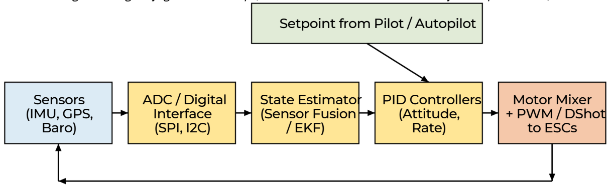
Figure 4: Digital flight-control loop (executed hundreds to thousands of times per second)
