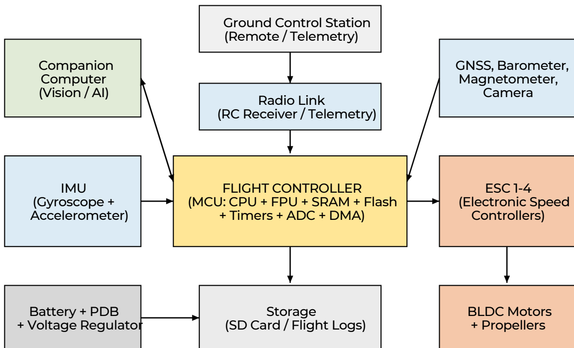
Figure 2: Computer organization of a typical quadcopter drone
