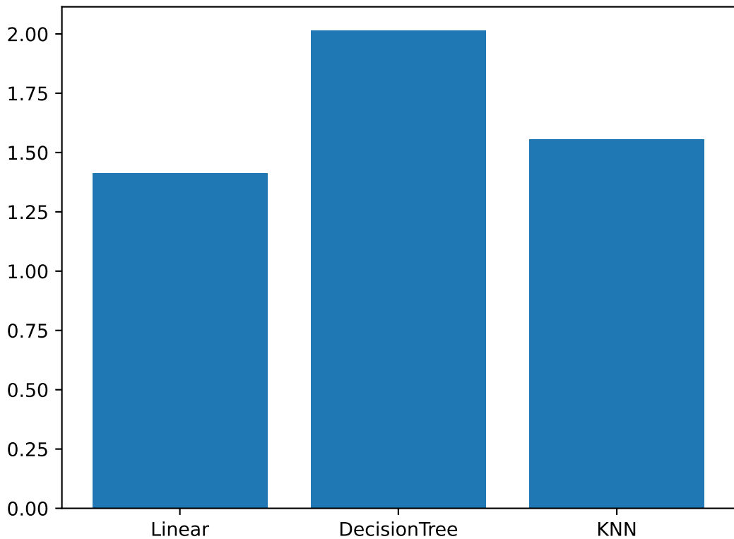
Baseline Models
