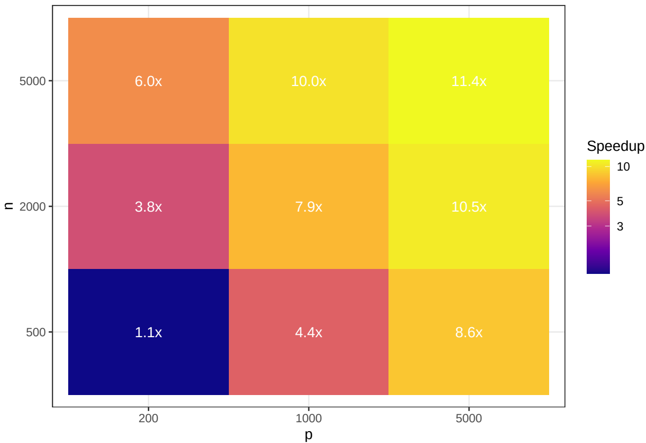
mfscreen2 speedup over mfscreen
