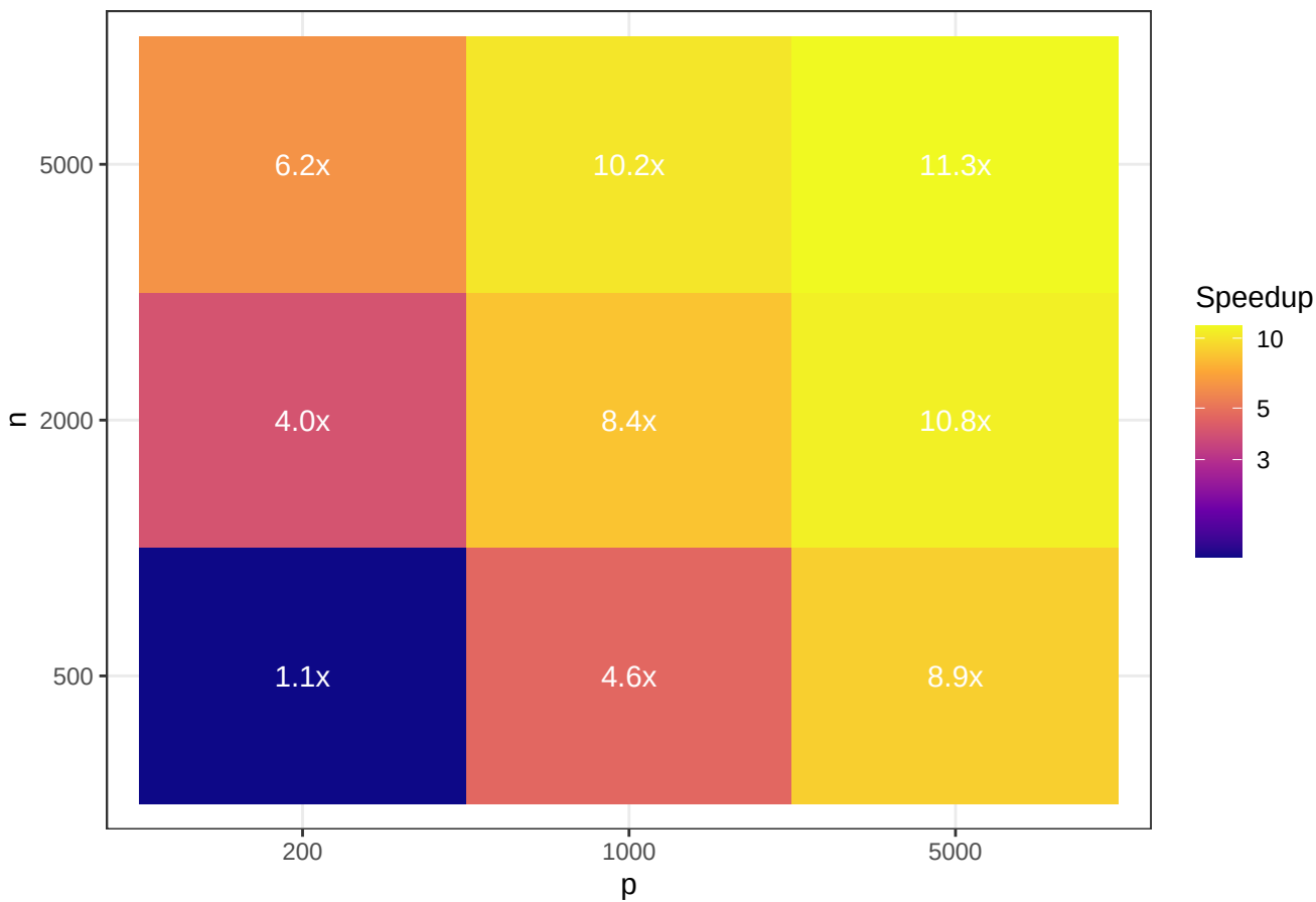
mfscreen speedup over mfscreen0
