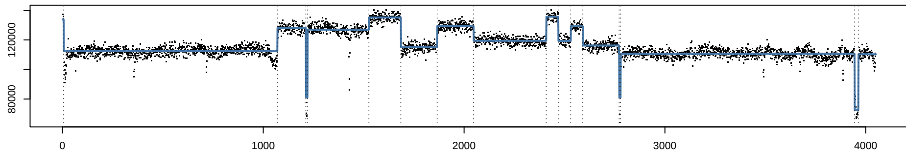
RFPOP reference
