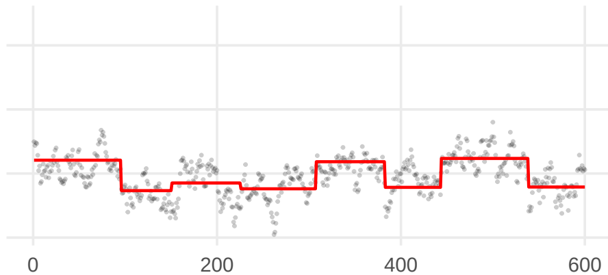
rand1
