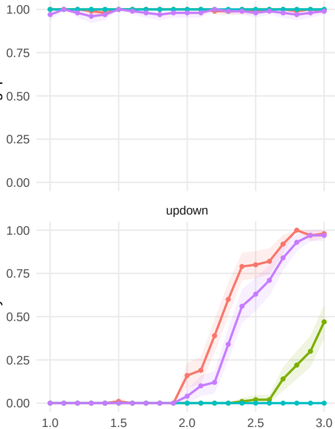
Probability of the correct number of changepoints
