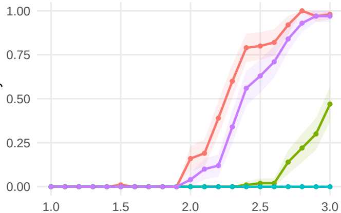
Probability of the correct number of changepoints
