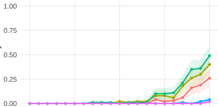
Probability of the correct number of changepoints
