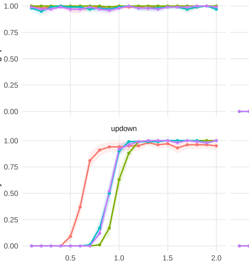
Probability of the correct number of changepoints
