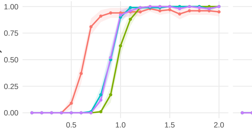
Probability of the correct number of changepoints
