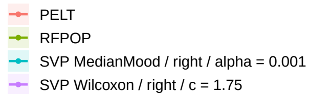
algorithm
