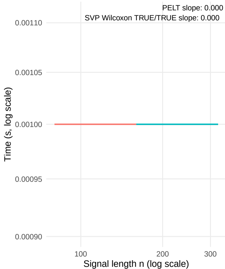
A. No changes: increasing n
