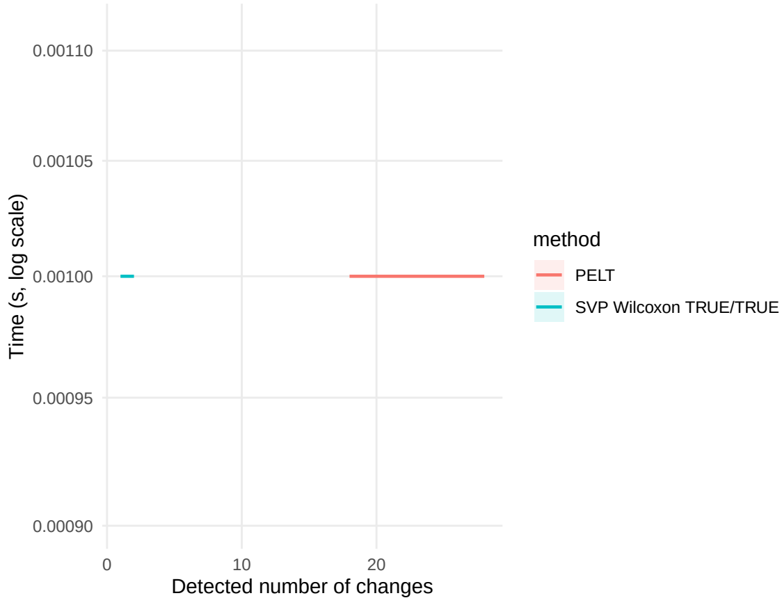
B. Fixed n: increasing changes
