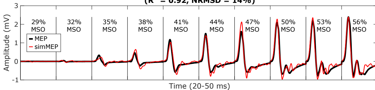
MEPs of subject 1 (R^2 = 0.92, \text{NRMSD} = 14\%)
