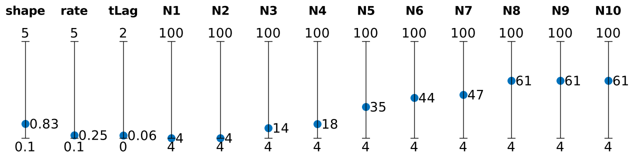
MEPs of subject 1 ( R^2 = 0.87 , NRMSD = 18%)
