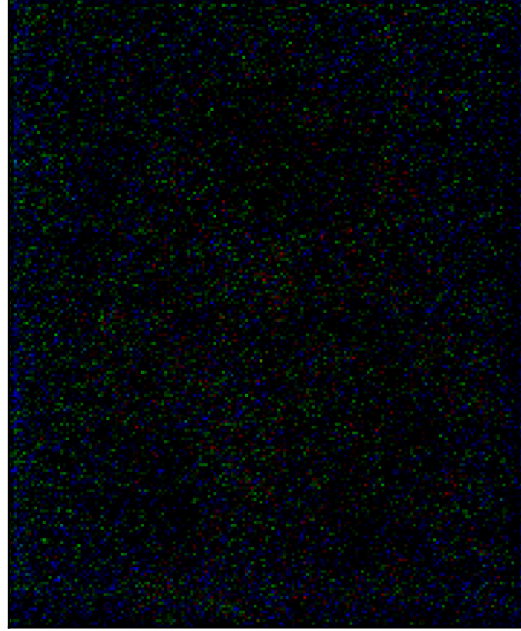
G_\theta(X_0, Z)
