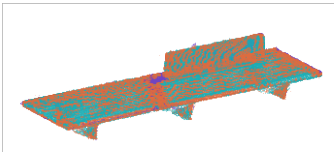
MASt3R-GA
