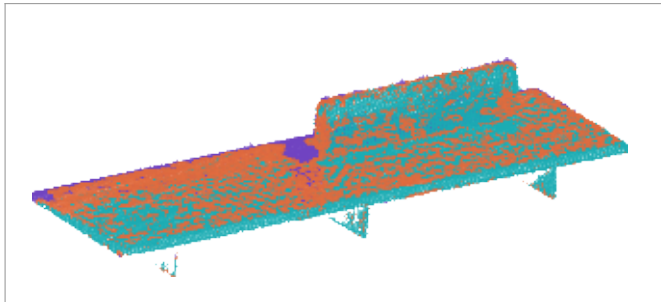
COLMAP
