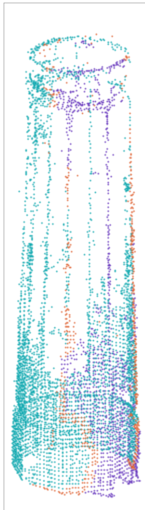
COLMAP
