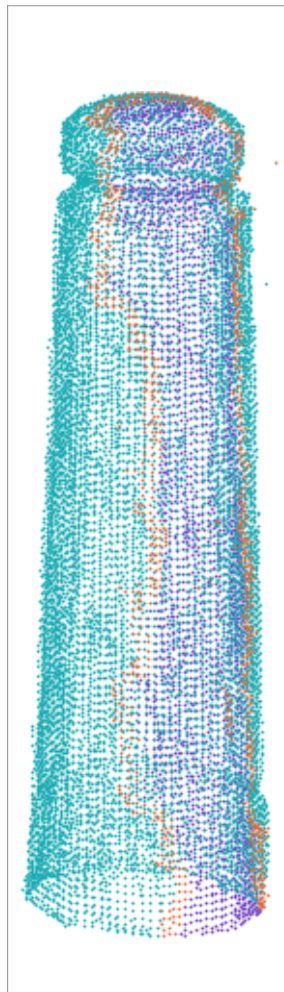
MASt3R-GA
