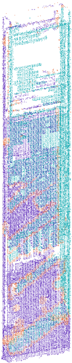
COLMAP
