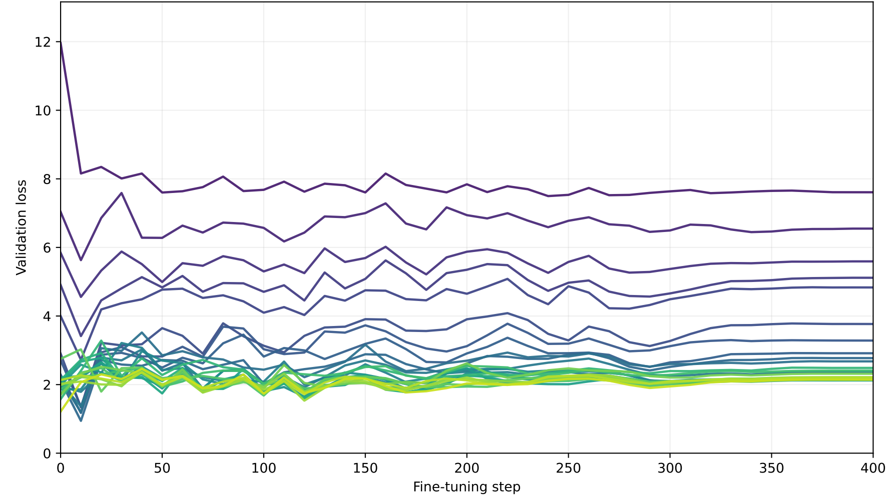
Clean validation loss
