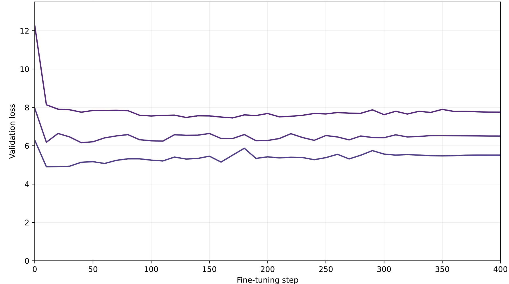
Clean validation loss
