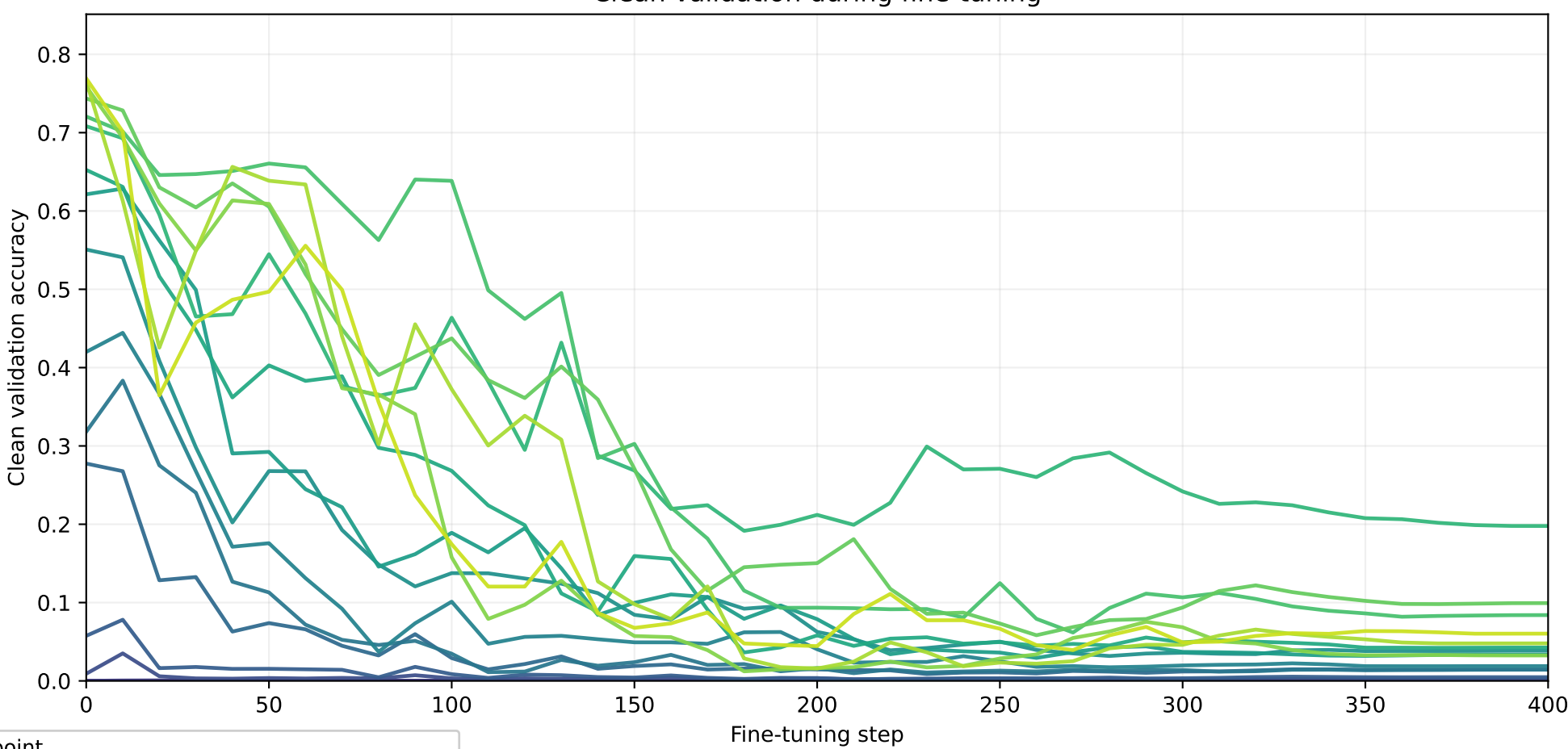
Clean validation during fine-tuning
