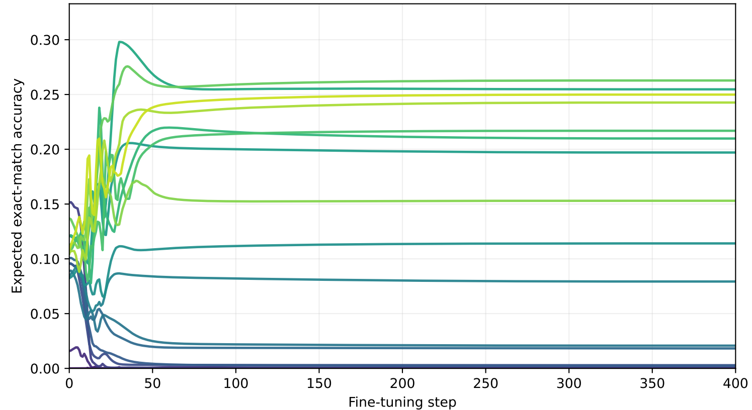
Clean validation accuracy during fine-tuning
