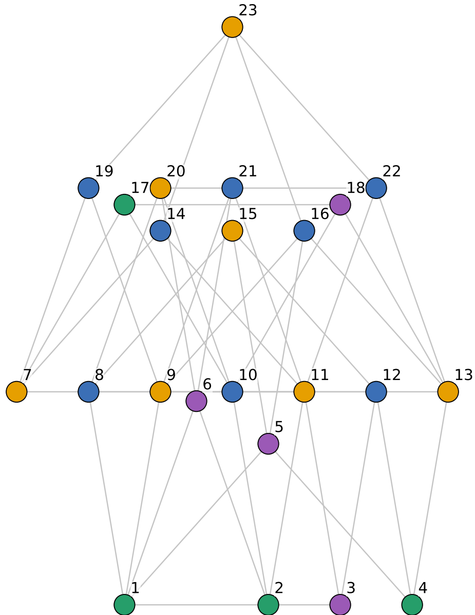
A proper four-coloring of G vertex colors: 0, 1, 2, 3
