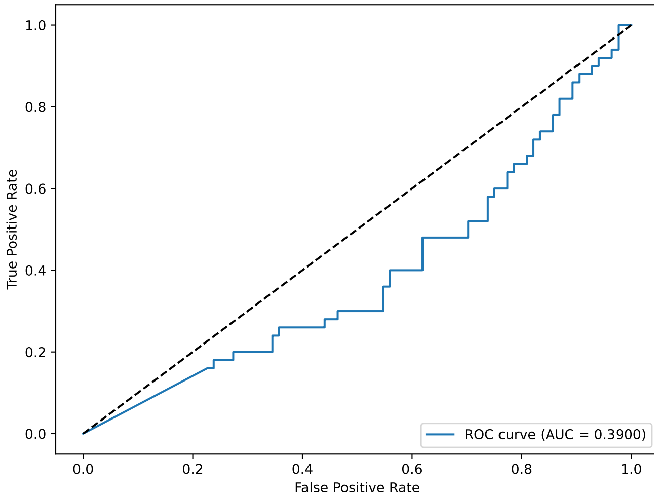
ROC Curve for PTB Prediction
