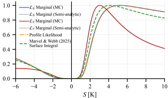
b Climate Sensitivity
