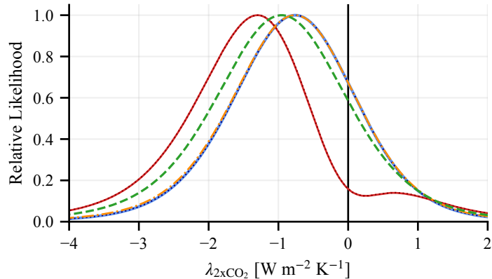
a Radiative Feedback
