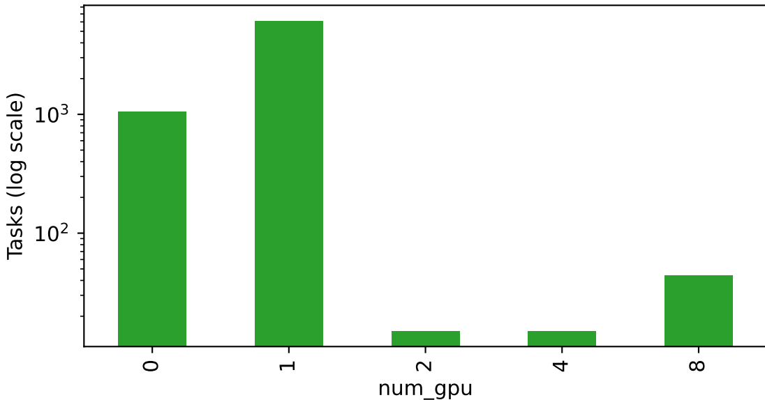
GPU demand distribution
