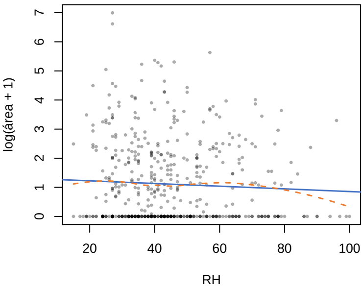
\log(\text{área}+1) \sim \text{RH}
