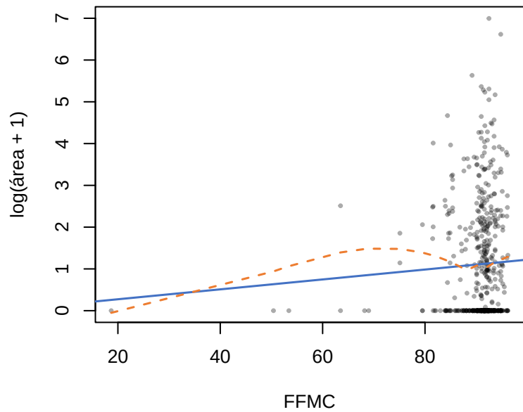
\log(\text{área}+1) \sim \text{FFMC}
