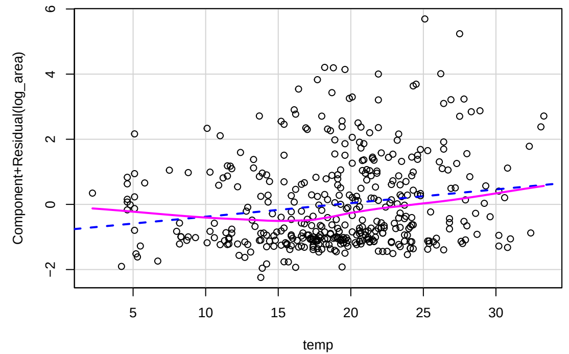
Figura 3: Residuos componente + residuo (crPlots)
