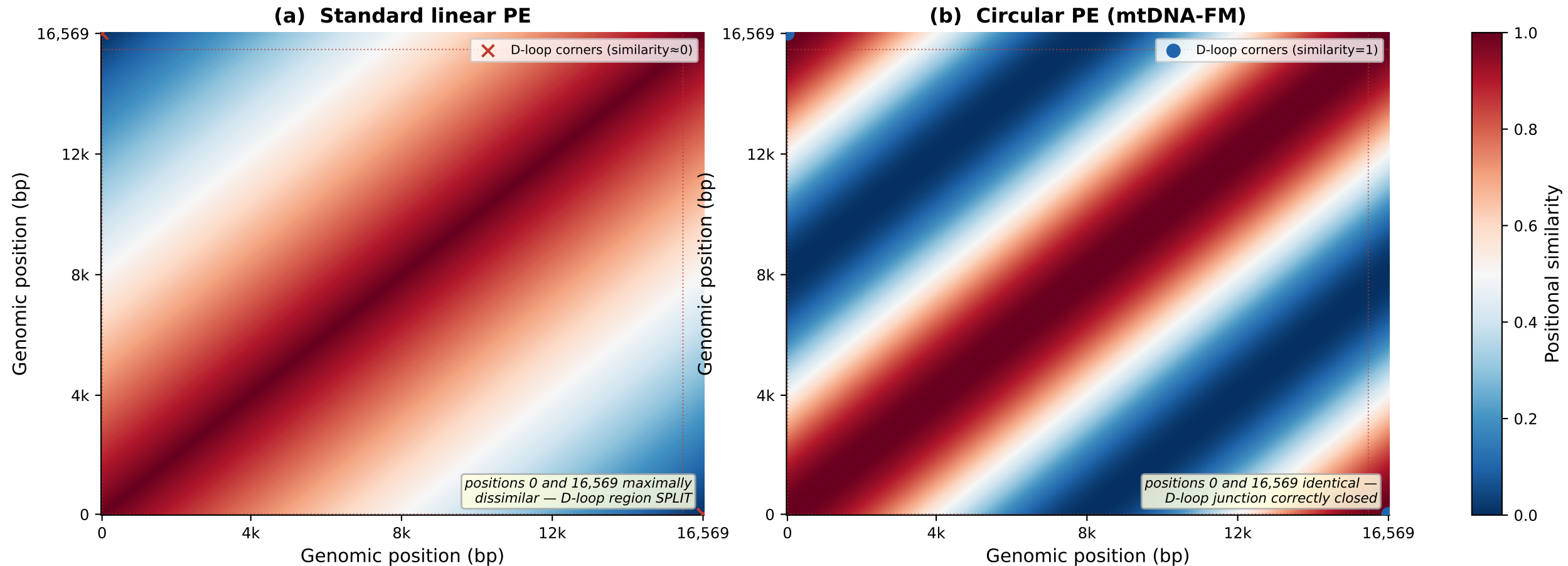
Figure 2: Positional similarity matrix — standard vs circular positional encoding Red dashed lines mark the D-loop region (positions 0 and ~16,024-16,569)
