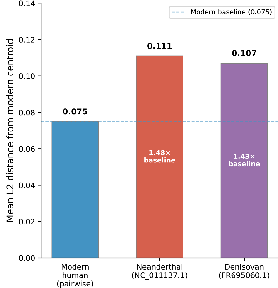
(b) Archaic sequence embedding distance (zero-shot; neither sequence in pre-training)
