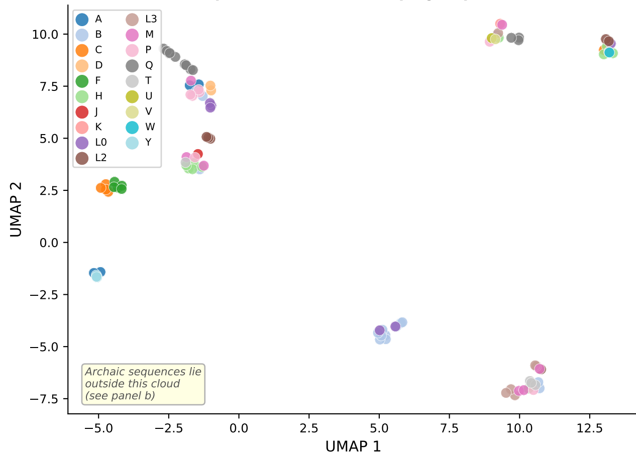
(a) Modern human mtDNA embedding space (100 sequences, zero-shot, haplogroup-coloured)
