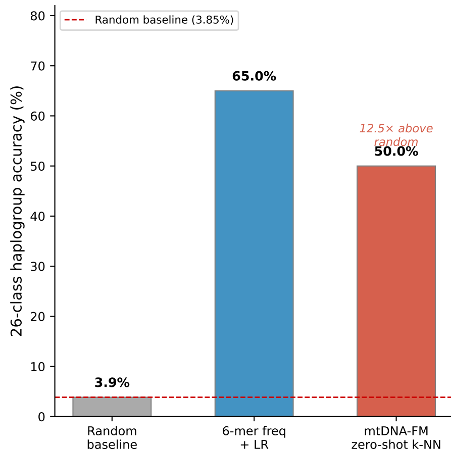
(b) Haplogroup classification (test set n = 1,263 )
