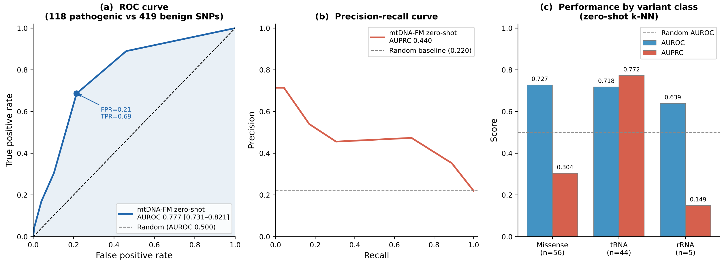
Figure 4: Zero-shot pathogenic variant discrimination (no pathogenicity labels in pre-training)
