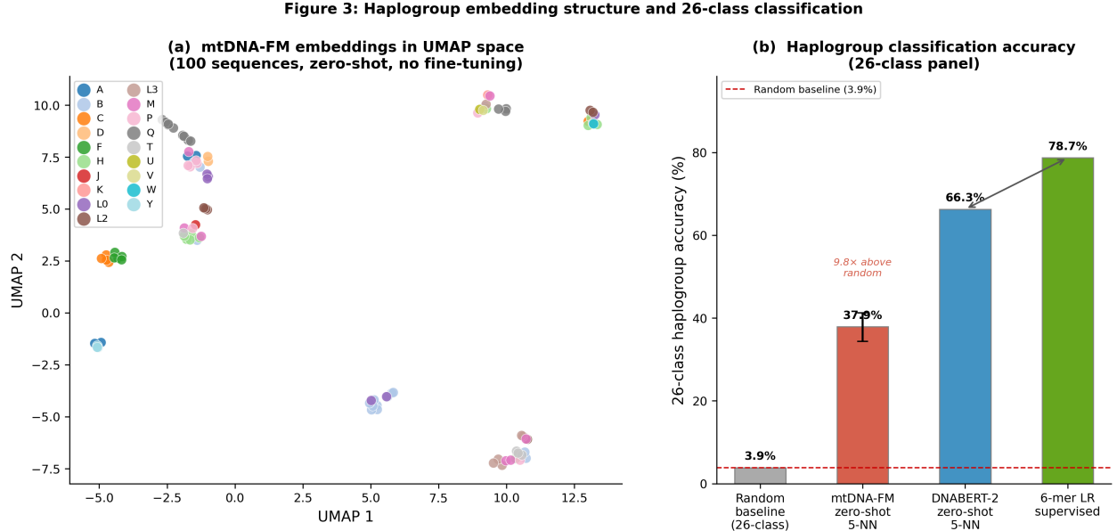
Figure 3: Haplogroup embedding structure and 26-class classification. (a) UMAP of MTDNA-FM embeddings for 100 sequences across 50 sub -haplogroups (used for visualization only; the classification task uses 26 major PhyloTree classes), coloured by major haplogroup. African L clades and the Asian M clade form separate regions without supervision; the West Eurasian haplogroups (H, HV, J, U, and relatives) overlap heavily, consistent with their near-zero classification F1 (Section 5.3). (b) 26-class haplogroup accuracy across four methods on the same 1,509/757 train/test split. Random baseline 3.85%; MTDNA-FM zero-shot 37.9% (9.8 \times above random; 95% CI shown); DNABERT-2 zero-shot 66.3%; supervised 6-mer logistic regression 78.7%. Neither MTDNA-FM nor DNABERT-2 used haplogroup labels.
