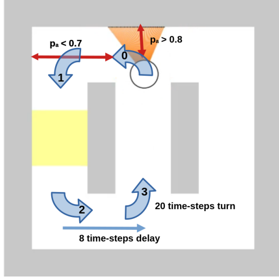
Figure 1: Illustrates the navigation implementation. The navigation is a loop made of 4 quarter-turns. - Turns 0, 1 and 2 are triggered by the wall ahead proximity. - Turn 3 is triggered by a delay after turn 2 and has a predefined precalibrated duration.
