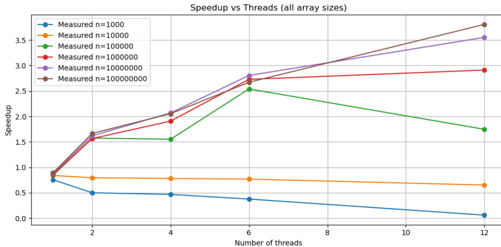
Σχήμα 9: Speedup vs threads for mergesort
