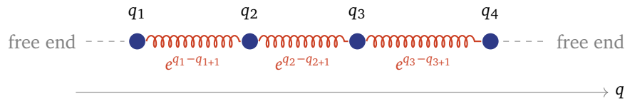
Figure 12.2: The open Toda chain, N = 4 . Neighbours interact through e^{q_n - q_{n+1}} , which is small while particle n is well behind particle n+1 and grows exponentially as it catches up. The end particles have one neighbour each.
