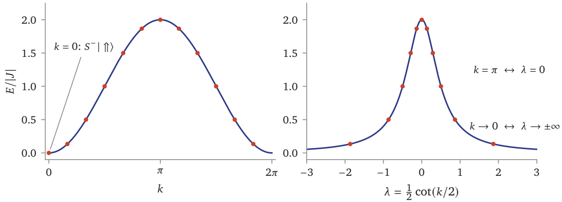
Figure 10.6: One magnon on a ring of N = 12 sites, for the ferromagnet J < 0 . Left: E = |J| (1 - \cos k) with the twelve allowed momenta; the dot at k = 0 is S^- |\uparrow\rangle , not a new state. Right: the same dots against the rapidity \lambda = \frac{1}{2} \cot(k/2) . The generator ( scripts/figures/magnon_dispersion.py ) asserts that the dots are the exact M = 1 spectrum.
