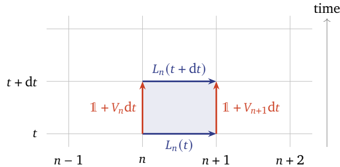
Figure 8.10: A plaquette of the space-time lattice. The two paths from lower left to upper right give (\mathbb{1} + V_{n+1} dt) L_n(t) and L_n(t+dt)(\mathbb{1} + V_n dt) ; zero curvature (8.23) says they agree to first order in dt .
