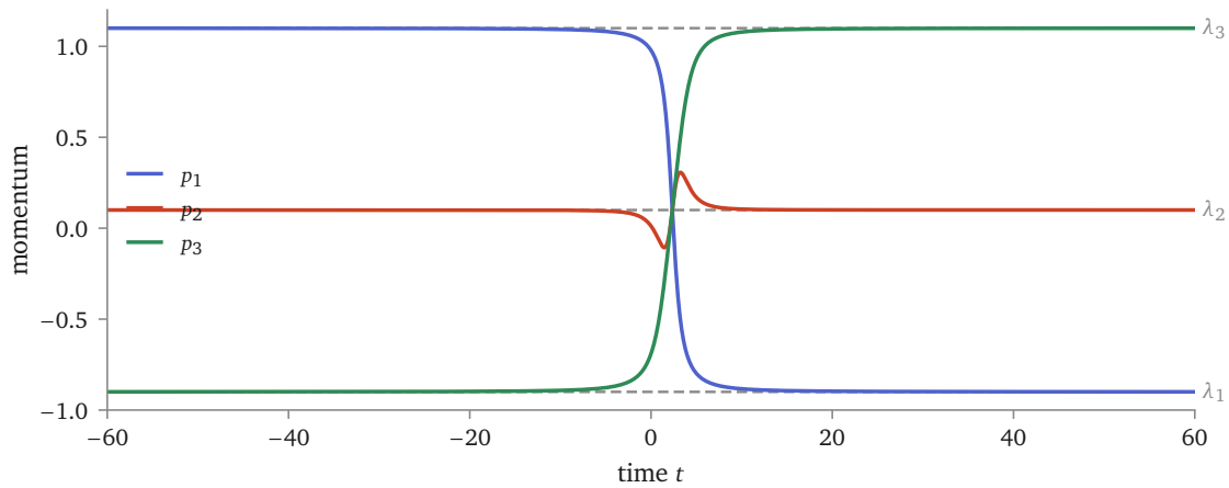
Figure B.5: Three particles of the rational gas, g = 1 : momenta (solid) and the eigenvalues of Moser’s L (dashed). The momenta are exchanged; the eigenvalues do not move ( scripts/figures/cm_scattering.py , which asserts the spectrum and the energy constant to 10^{-9} and both asymptotic orders).
