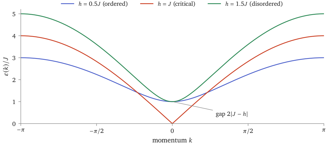
Figure 14.4: The quasiparticle energy (14.15) below, at and above the critical field. Its minimum, at k = 0 , is 2|J - h| , the same for h = 0.5J and h = 1.5J ; at h = J it closes linearly. (scripts/figures/tfim_dispersion.py.)
