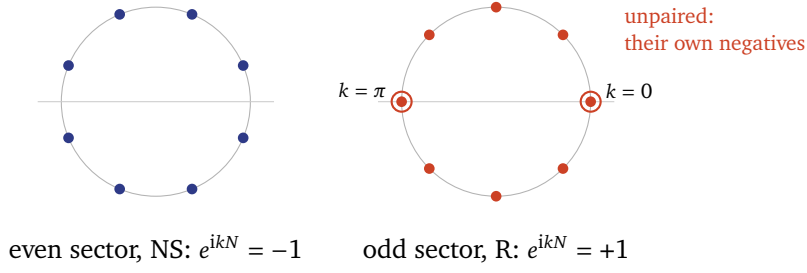
Figure 14.2: The two grids of momenta for N = 8 , drawn as e^{ik} on the unit circle. Each point is paired with its mirror image -k . The R grid has two points on the real axis, k = 0 and k = \pi , that pair with nothing; the NS grid has none.
