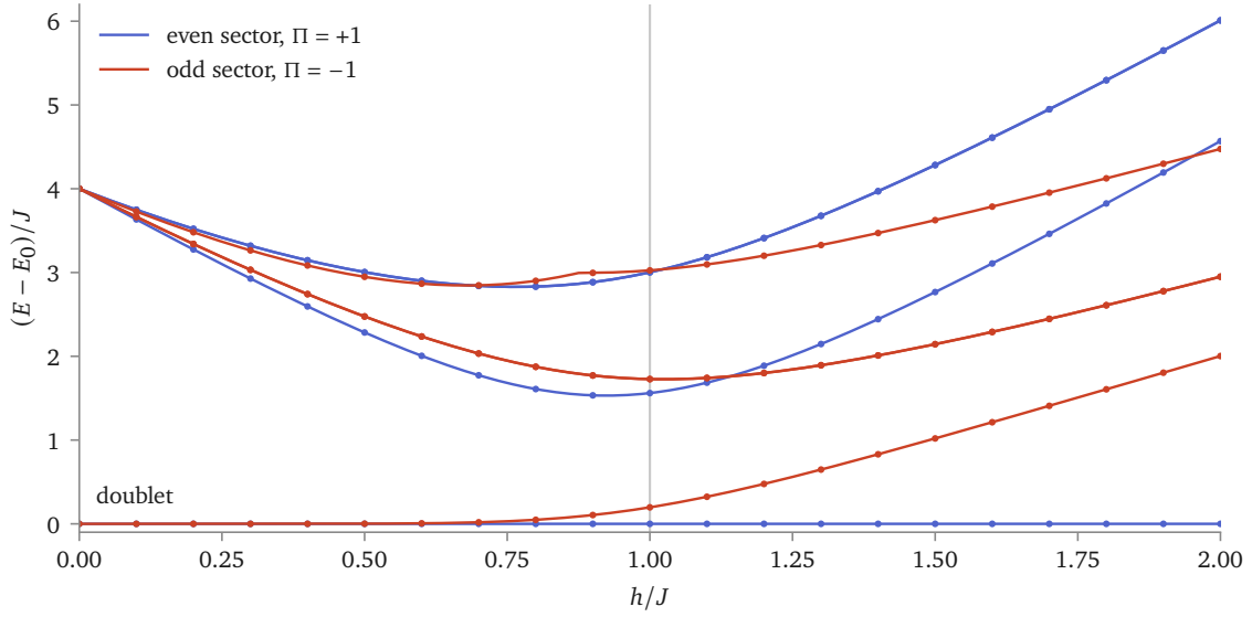
Figure 14.3: The lowest levels of each parity sector of the TFIM, N = 8 , from the ground energy. Lines: Theorem 14.6; dots: exact diagonalisation. The generator ( scripts/figures/tfim_spectrum.py ) asserts agreement of each sector's whole spectrum to 10^{-9} at every dotted field. Levels at \pm k coincide.
