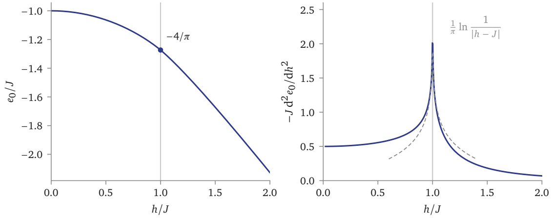
Figure 14.5: Left: the ground-state energy per site (14.22); it looks smooth. Right: minus its second derivative, which diverges at h = J , with the asymptote \frac{1}{\pi} \ln \frac{1}{|h-J|} (dashed, J = 1 ). The generator asserts the slope 1/\pi to 3% on both sides.
