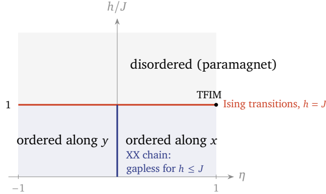
Figure 14.6: The XY chain’s phase diagram in the plane of anisotropy \eta and field h/J . The gap closes on the line h = J and on the segment \eta = 0 , h \leq J ; elsewhere it is open. The TFIM is the edge \eta = 1 ; the transverse-field transition of this lecture is the dot. (A finer line inside the ordered phases, where correlations change their manner of decay, is omitted.)
