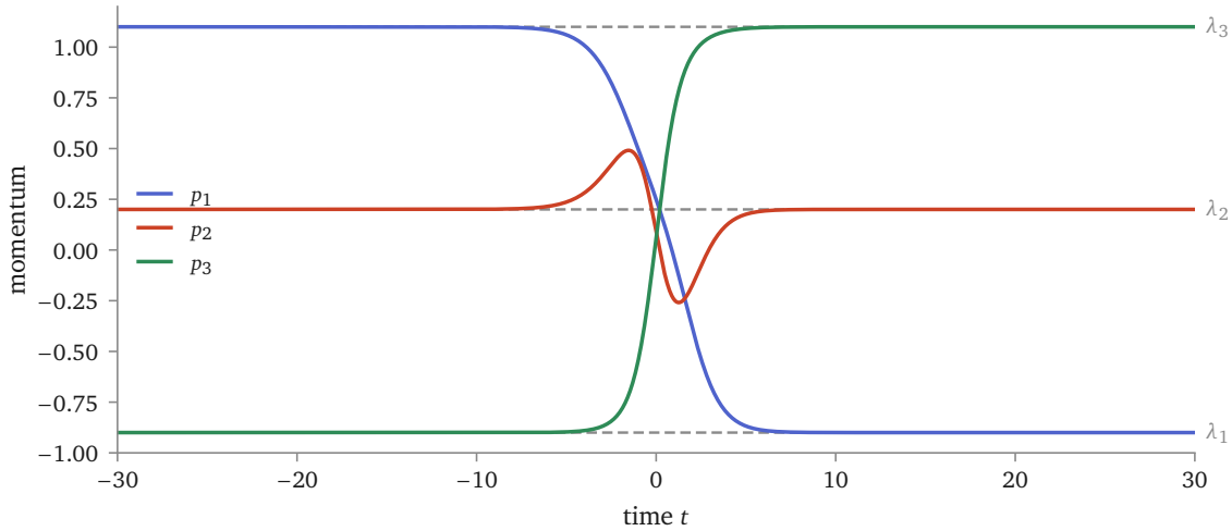
Figure 12.4: Three particles scatter. Their momenta (solid) start on the eigenvalues of L (dashed) in decreasing order and end on them in increasing order; in between, the eigenvalues do not move (scripts/figures/toda_scattering.py, which asserts the spectrum constant to 10^{-9} and both limits).
