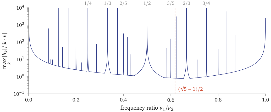
Figure 7.1: Small denominators for the rotors of Example 7.1, V = P_r P_r , r = \frac{1}{2} : the largest term |h_k| / |k \cdot \nu| of (7.4), |k_1| + |k_2| \leq 40 , against the frequency ratio. The low-order rationals show as spikes; the truncated sum has a pole at every rational a/b with a + b \leq 40 , of width shrinking like r^{a+b} . Most of the line stays low (scripts/figures/small_denominators.py).
