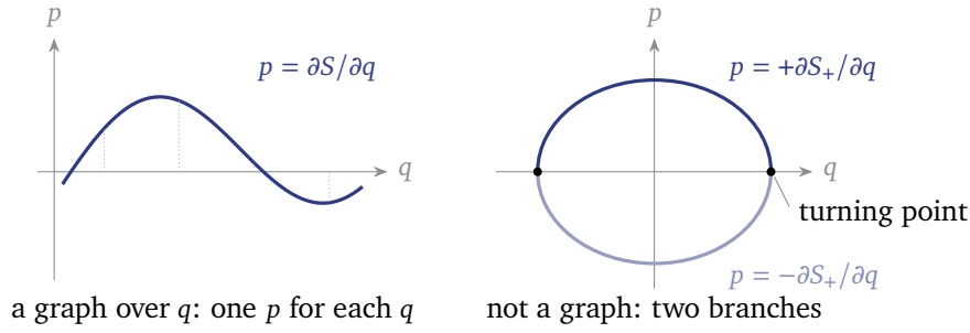
Figure 3.6: Left: the graph of dS , Lagrangian for every S (Proposition 3.25). Right: an oscillator orbit, Lagrangian by Example 3.23 but not a graph — two points over each q , and a vertical tangent at the turning points. Each branch is a graph, generated by \pm S_+ ; the turning points are where Lecture 5's S(q, I) changes branch.
