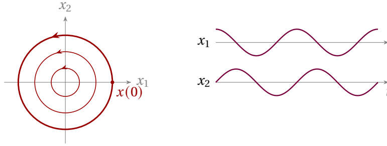
Figure 4: Phase portrait of the system \dot{x} = Ax for A = \begin{pmatrix} 0 & -\omega \\ \omega & 0 \end{pmatrix} : every trajectory is a circle traversed counterclockwise. The highlighted trajectory starts at the point x(0) = (1, 0) ; its coordinates x_1(t) = \cos \omega t and x_2(t) = \sin \omega t oscillate harmonically.
