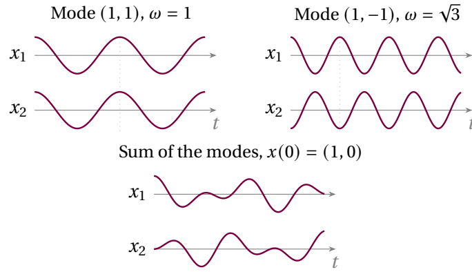
Figure 3: The normal modes of two coupled masses: the displacements x_1(t) and x_2(t) of the masses. In the mode (1, 1) the masses oscillate together, x_1 = x_2 = \cos t . In the mode (1, -1) they oscillate in opposite directions, x_1 = -x_2 = \cos \sqrt{3} t . The dotted line marks the moment when x_1 is back at its maximum. The sum of the modes for x(0) = (1, 0) and \dot{x}(0) = 0 : the oscillation passes from the first mass to the second and back.
