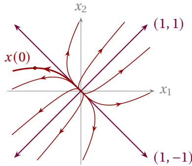
Figure 2: Phase portrait of the system \dot{x} = Ax for A = \begin{pmatrix} 2 & 1 \\ 1 & 2 \end{pmatrix} . Each curve is the trajectory of one initial state, and the arrow shows the direction of motion. The highlighted trajectory passes through the point x(0) = (-2, 1) .
