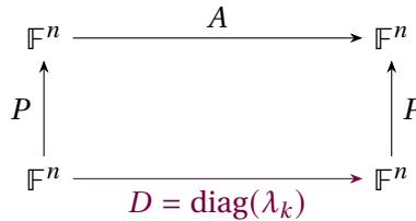
Figure 1: In the eigenbasis the operator is represented by the diagonal matrix D . The change of basis P gives A = PDP^{-1} . Powers and functions are applied to the diagonal entries of D .
