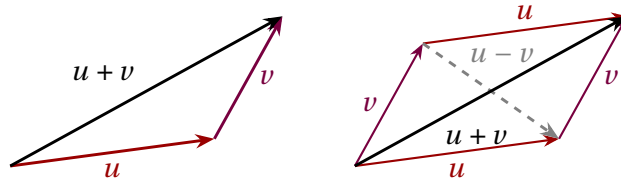
Figure 2: Left: the triangle inequality. The direct path u + v is no longer than the two sides u and v : \|u + v\| \leq \|u\| + \|v\| . Right: the parallelogram law. The squares of the two diagonals u + v and u - v add up to the squares of the four sides: \|u + v\|^2 + \|u - v\|^2 = 2\|u\|^2 + 2\|v\|^2 .
